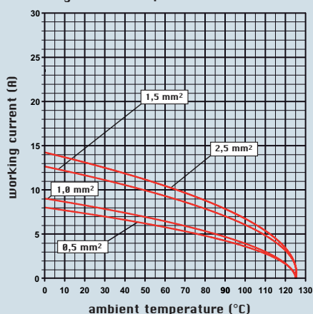
diagram CDSH 42 poles
